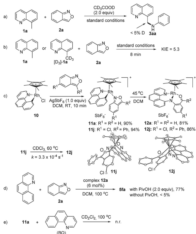
Scheme 6. Mechanistic studies. [24]
